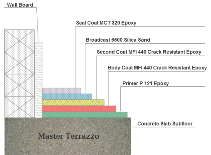
Installation Diagram MasterFlex Industrial 1/8"
