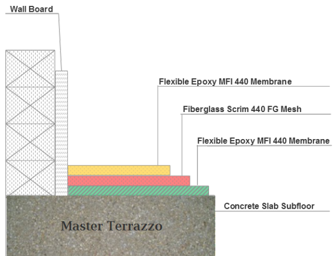
Installation Diagram MasterFlex Flexible Epoxy Under Flooring 40 Mils
