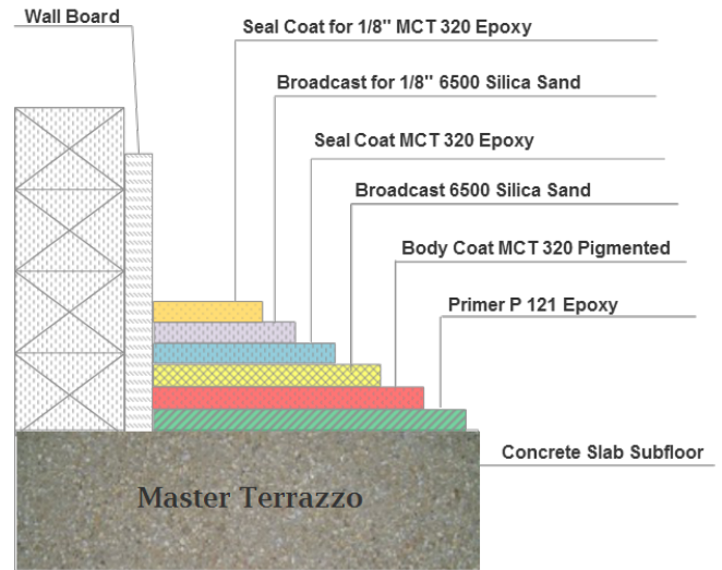
Installation Diagram Morricite MasterTrac Broadcast 1/16" or 1/8"
