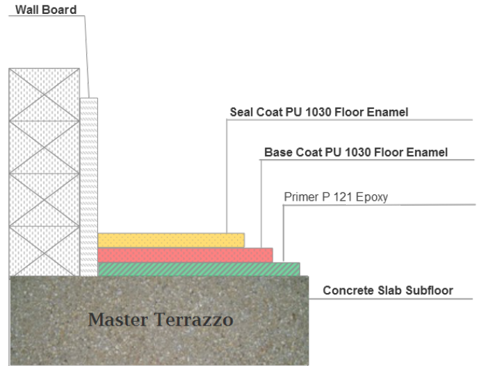
Installation Diagram MasterShield Industrial Flooring & Aircraft Hangar
