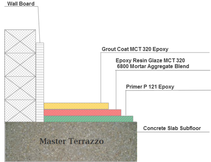
Installation Diagram MasterShield SS 3/16"-1/4" Topping
