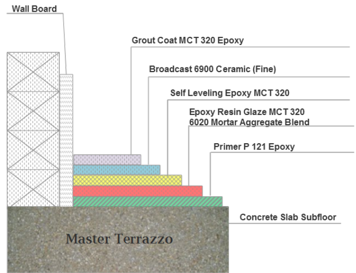
Installation Diagram MasterShield U11 (3/16" Topping)
