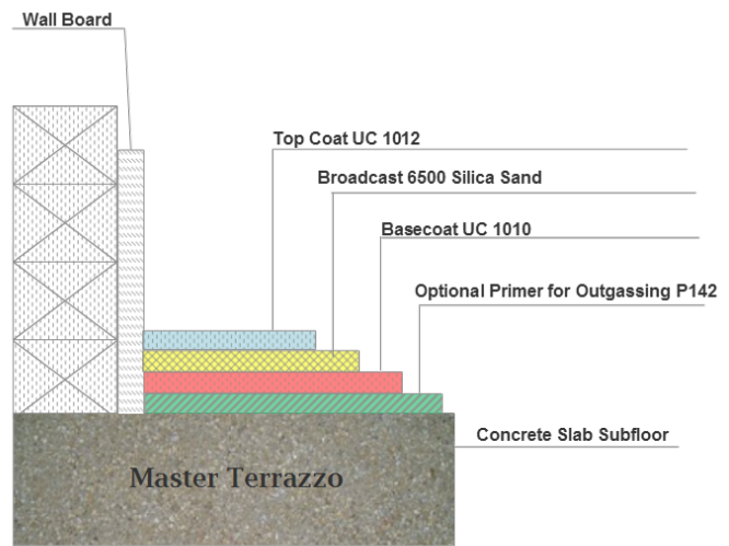
Installation Diagram UC 10101 S
